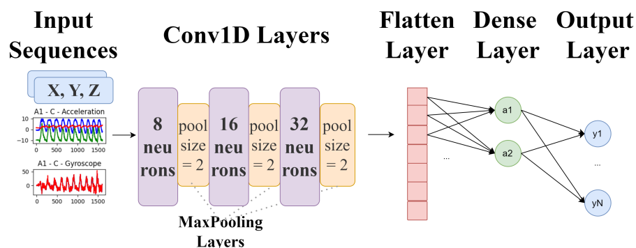
Figure 6. CNN model definition showing the included layers.
