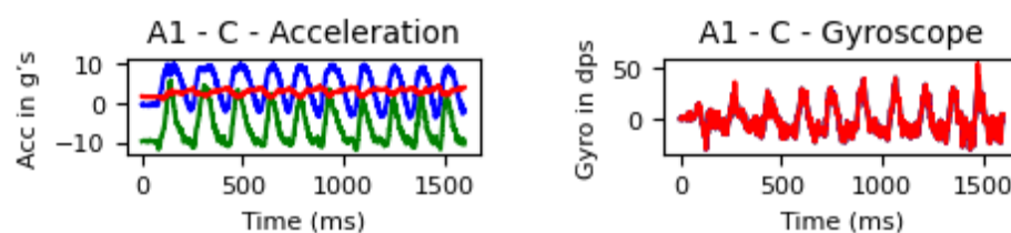
Figure 4. Signal acquired on the Bicep Curl exercise by the accelerometer (title Acceleration) and the gyroscope (title Gyroscope) from the 1 subject (X values in blue, Y in green, and Z in red).
