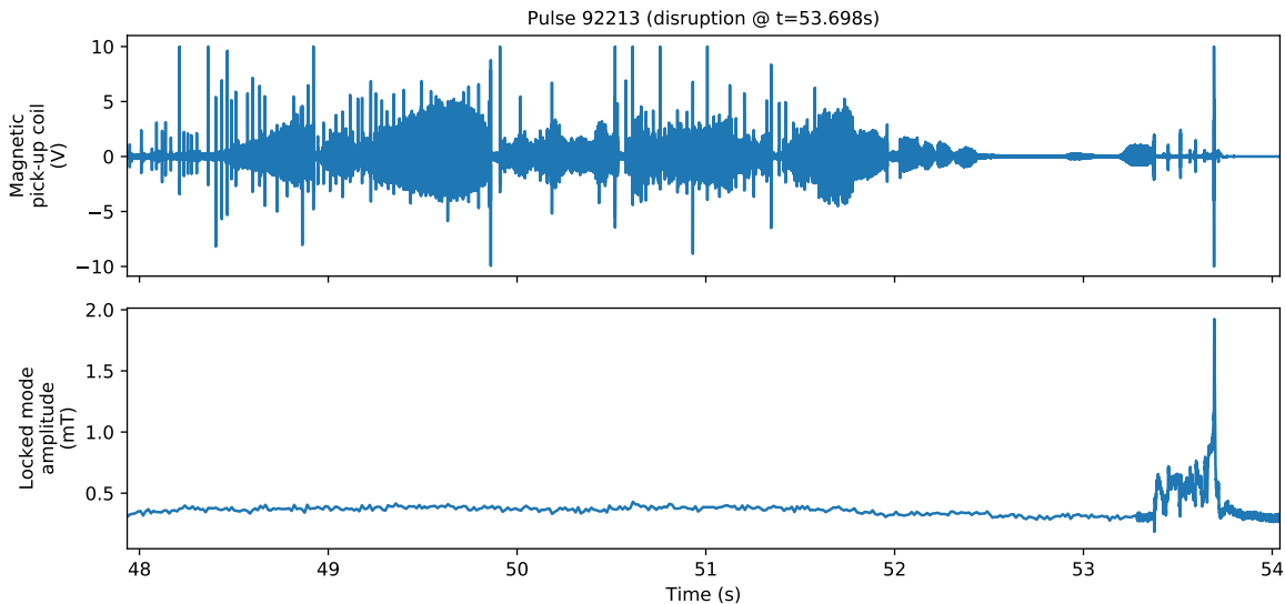
Figure 2. Magnetic pick-up coil ( top ) and locked mode amplitude ( bottom ) signals for JET pulse 92213 from t=48 s to t=54 s.
