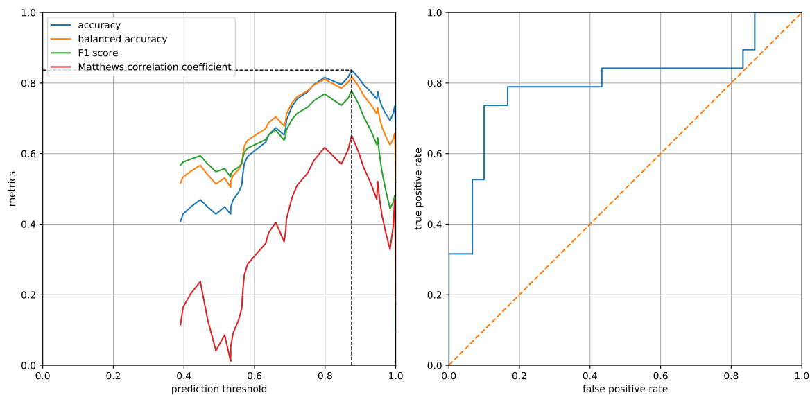
Figure 9. Classification metrics and ROC curve for a variable threshold on model output. Results are shown for the 10% of pulses in the validation set (49 pulses).
