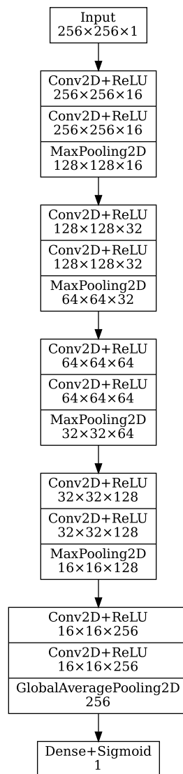
Figure 4. Convolutional neural network to predict the occurrence of a locked mode from a 256 \times 256 image drawn from an MHD spectrogram.
