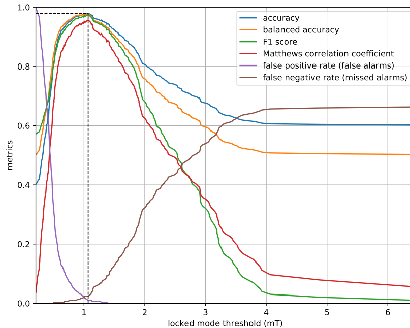
Figure 3. Binary classification metrics for disruption prediction with a threshold on the locked mode amplitude, for a dataset of 485 baseline pulses.
