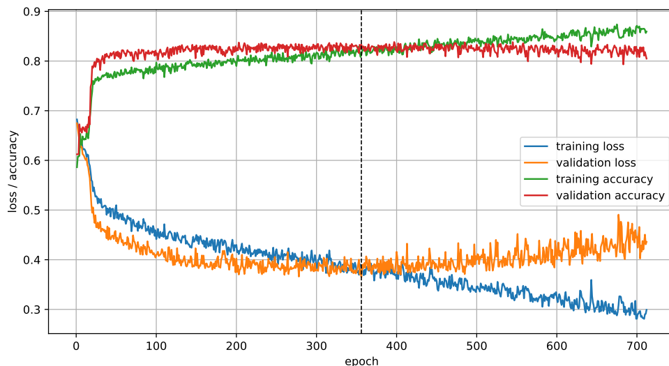
Figure 5. Loss and accuracy during the training process. The dash line indicates the point at which the minimum validation loss was achieved.
