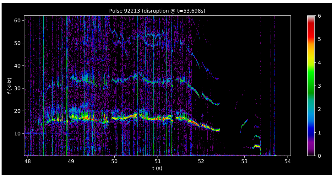
Figure 1. MHD spectrogram for JET pulse 92213 from t = 48\text{s} to t = 54\text{s} . The spectrogram is plotted with logarithmic amplitude, so the color intensities have arbitrary units.
