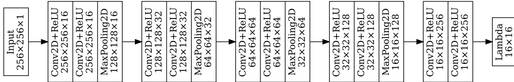
Figure 7. Model used to generate the class activation map for a given input image.
