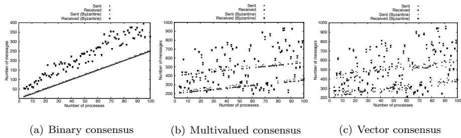
Figure 3: Messages exchanged in a network with 4 – 100 processes.
