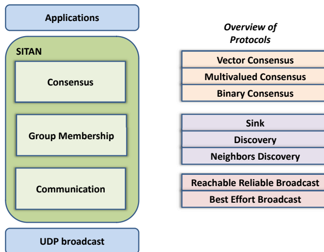
Figure 1: SITAN protocol stack
