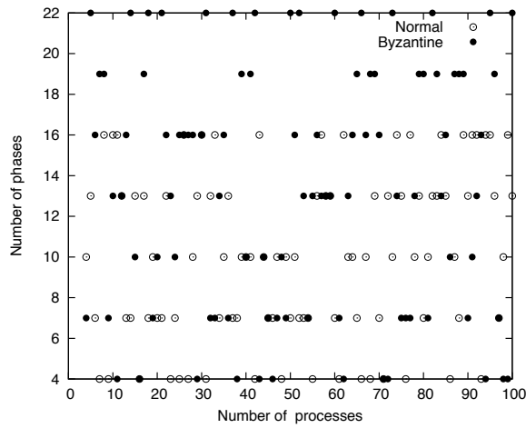
Figure 4: Number of phases to achieve Binary Consensus
