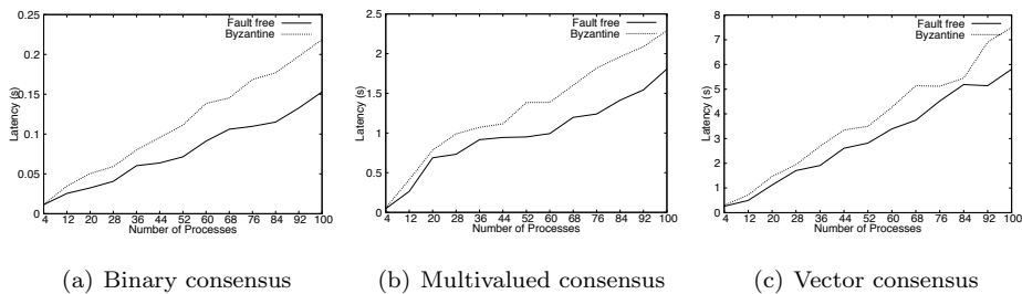
Figure 2: Consensus latency in both fault-free and Byzantine scenarios.
