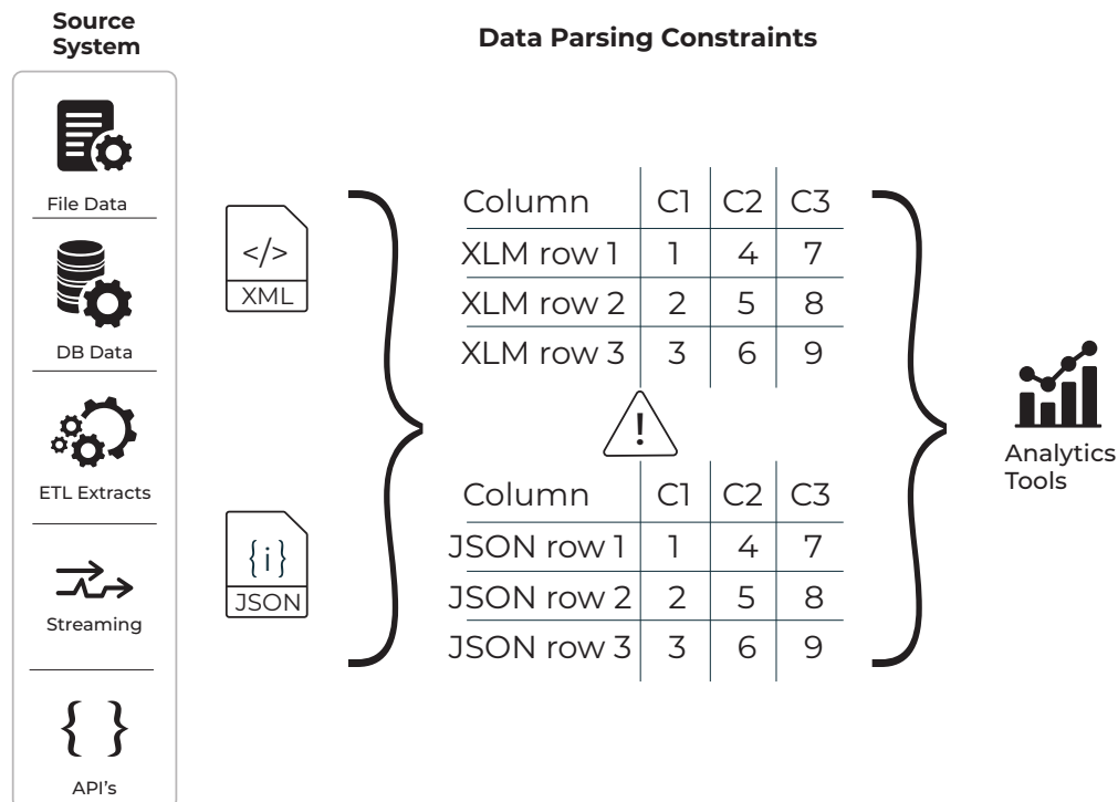
Figure 1: Simple data parsing representation using Unicage. It is possible to acquire data from different sources and file formats, for example XML or JSON, and then parse it using the Unicage tools to obtain uniform and ready-to-use data for analytic tools, databases or other software.
