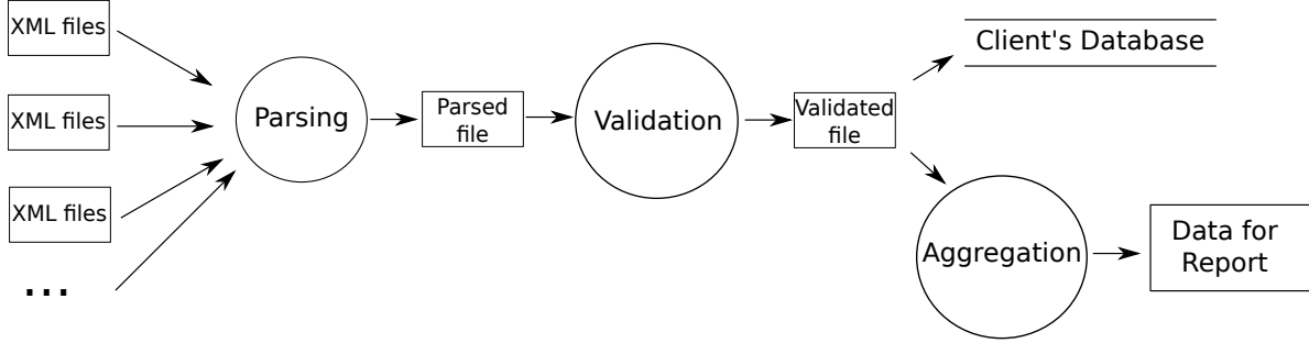
Figure 3: Data-flow representation of the solution comprising 3 scripts that perform the steps required by the use case: parsing, validation, and aggregation.
