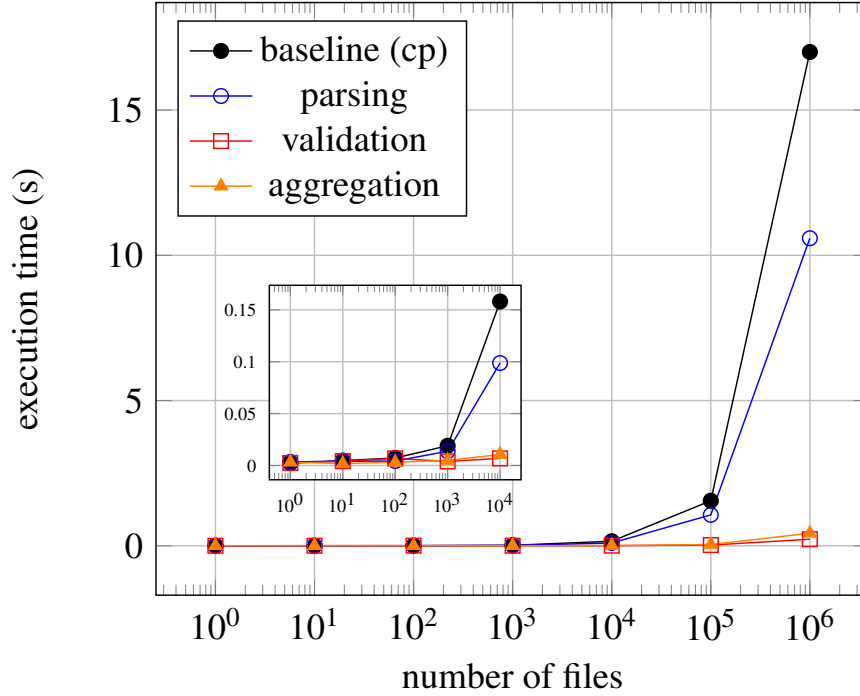
Figure 4: Comparison between the execution time of the different parts from our solution with the copy command (baseline)
