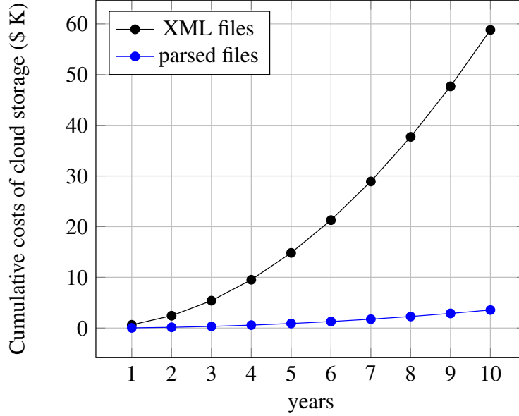
Figure 5: Estimate of cumulative costs of cloud storage per year. Using the notation of Eq. 1, \alpha = \$0.01 , D = 810 for the XML files and D = 49 for the parsed data.
