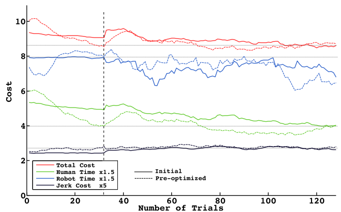
Fig. 6. Components of the cost function for the two conditions of Exp. A averaged across all subjects.
