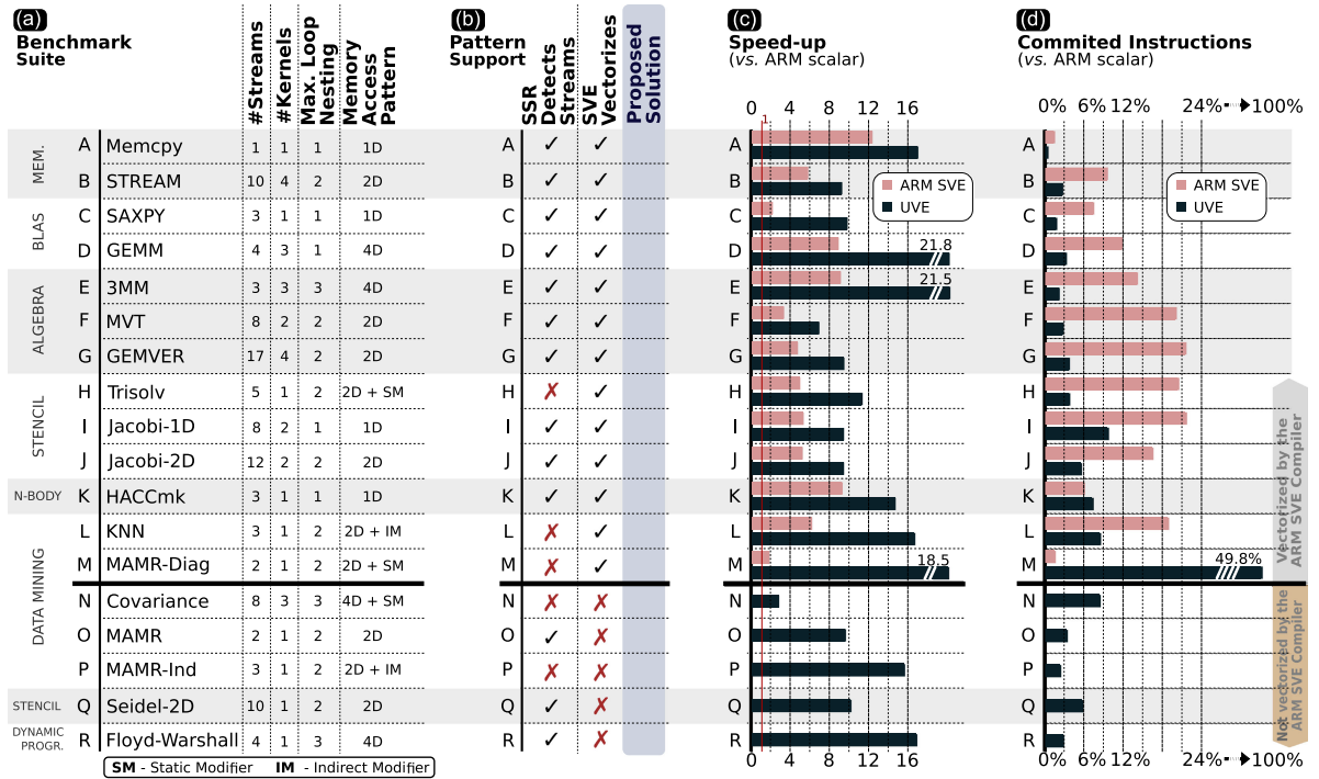
FIGURE 5. Characterization of the adopted benchmark set regarding (a) loop structure and memory access pattern, (b) SSR stream detection and SVE vectorization coverage, (c) UVE performance, and (d) code reductions (measured in number of committed instructions during execution).
