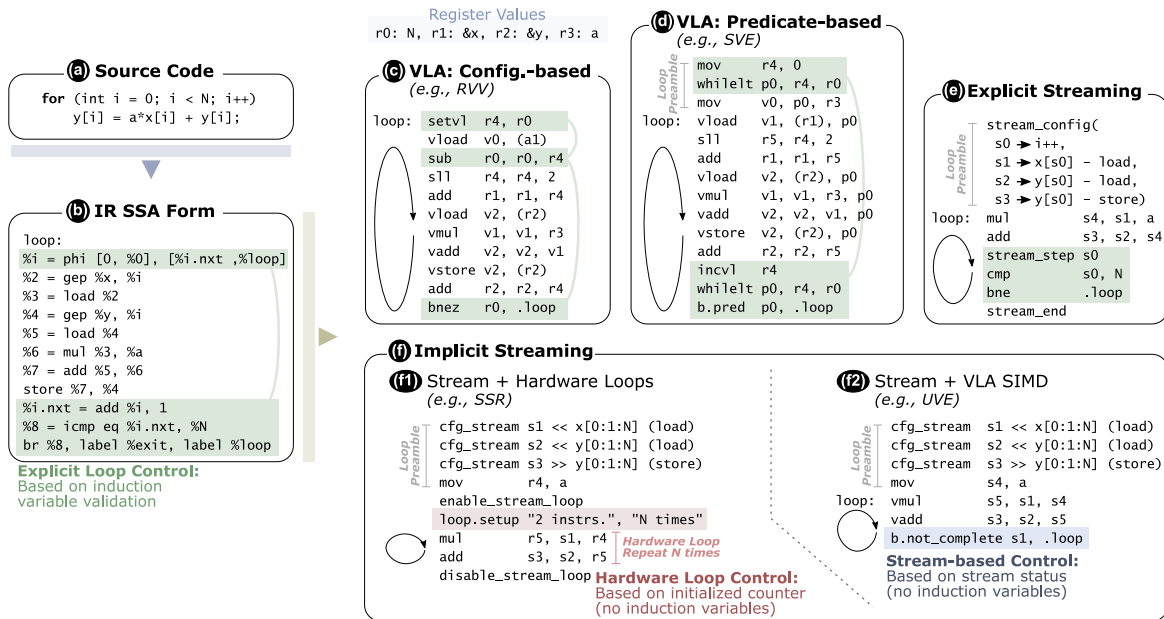
FIGURE 1. Representation of the saxpy kernel in (a) C code and (b) LLVM IR format; in VLA SIMD extensions pseudoassembly based on (c) vector length configuration and (d) loop predication; and pseudoassembly stream-based extensions with (e) explicit and (f) implicit stream iteration [(f1) using hardware loops and (f2) with stream vectors]. Note the presence of the induction variable exposed in (b) in examples (c), (d), and (e) and its implicit elimination in (f).
