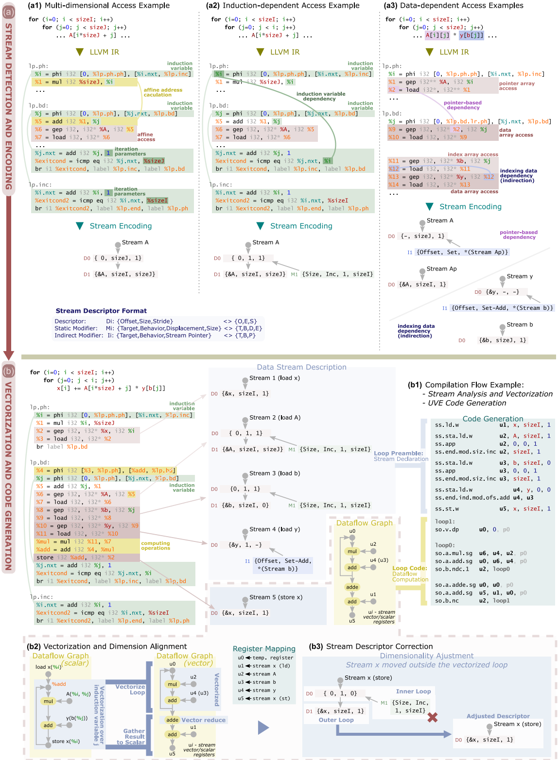
FIGURE 3. Illustration of each step of the LLVM IR pass that implements our proposed compilation flow, including depictions of (a) the memory access pattern detection (multidimensional, induction-, and data-dependent) and stream encoding schemes; and (b) the vectorization and code generation procedures.
