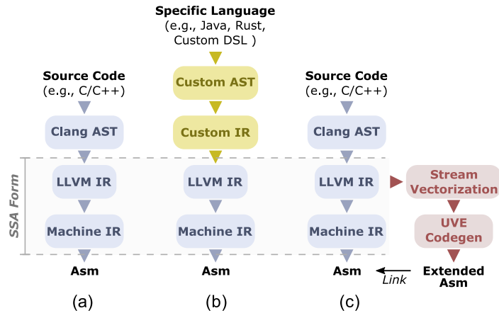
FIGURE 2. Typical compilation flows for (a) the base LLVM infrastructure, (b) LLVM-based custom compilers, and (c) the proposed compilation flow.
