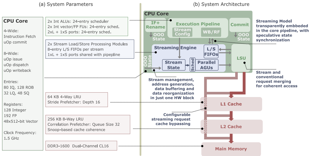
FIGURE 4. System overview, depicting (a) the system model configuration parameters (based on public information about the ARM Cortex A76, and both 1,7 ), and (b) the system architecture featuring the UVE Streaming Engine embedded in an out-of-order core and its connections to the memory hierarchy. The Streaming Engine parameters are specific for UVE, with the remaining being common to UVE, baseline (ARM), and SVE.
