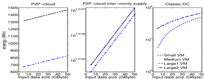
Figure 3: Energy consumption for various inputs across scenarios
