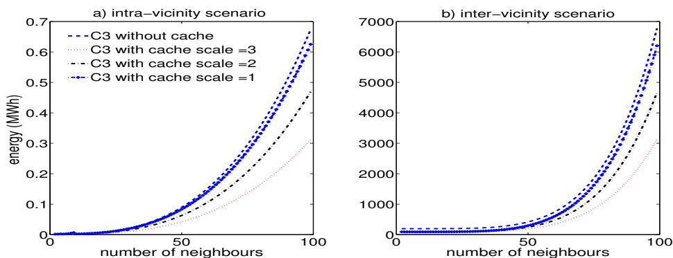
Figure 8: Impact of cache scale in energy consumption
