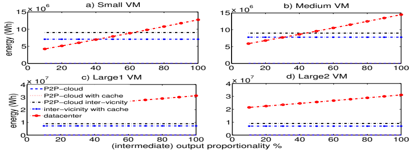
Figure 5: Energy consumption of a 5GB input application running on different VMs across scenarios
