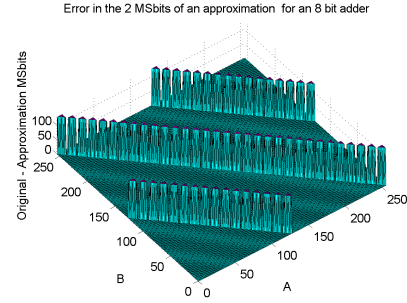
Fig. 5. Difference in the MSBs between the detection approximation and the expected result for an 8-bit adder (Hamming distance).
