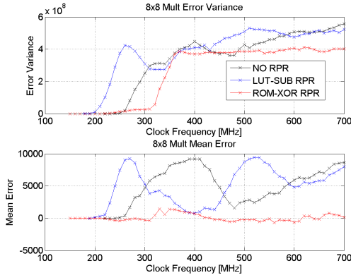
Fig. 8. Error variance and mean error at the output of an 8-bit bit unsigned LUT-based multipliers at different clock frequencies.
