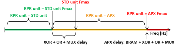
Fig. 4. Illustration of the maximum clock frequencies, and delays, for standard and proposed RPR units and their operating regimes: error-free/expected result (green), error-prone/approximated result (orange) and incorrect result (red).
