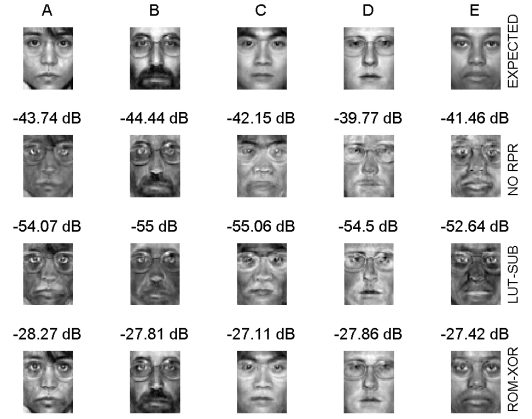
Fig. 9. Reconstructed faces (A-E) in the original space without timing errors (EXPECTED), and computed from the projections collected from implementations of different multipliers architectures (NO RPR, LUT-SUB RPR, ROM-XOR RPR) at 270 MHz. On top of each face there's the corresponding reconstruction error.
