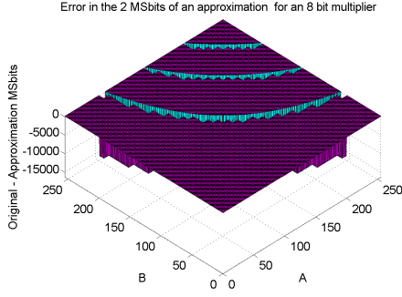
Fig. 6. Difference between a detection approximation and the expected MSbits at the output of the multiplier.
