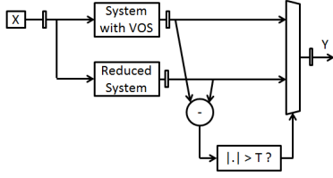
Fig. 2. Typical RPR architecture applied to a system.
