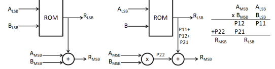
Fig. 1. ROM-based fast adder (left) and multiplier (right).
