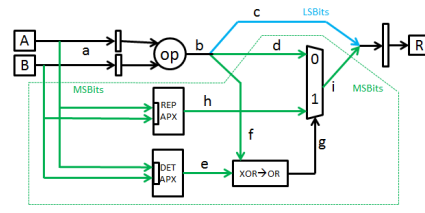
Fig. 3. Proposed RPR architecture applied to a generic combinational operator.
