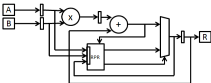
Fig. 7. Diagram of a rolled multiply-accumulate circuit with RPR.
