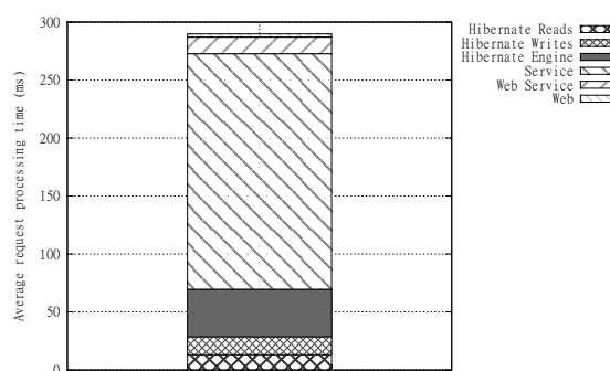
Figure 6: Request processing time breakdown.
