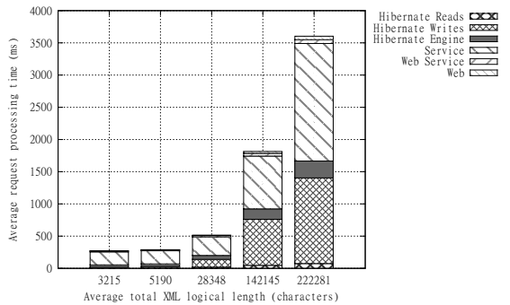
Figure 8: Request processing breakdown for increasing SOAP size.
