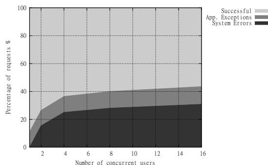
Figure 13: Outcome of requests for increasing concurrent users.
