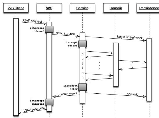
Figure 2: Sequence diagram of STEP Web Service.
