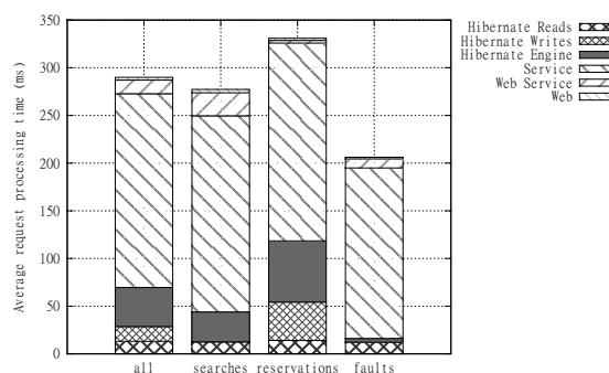
Figure 7: Request processing breakdown for different request types.
