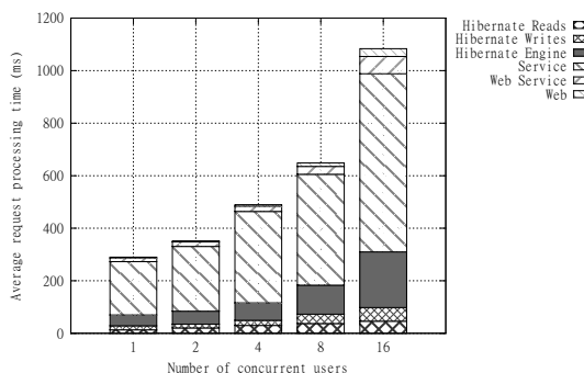
Figure 12: Request processing breakdown for increasing concurrent users.
