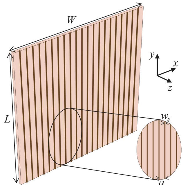
Fig. 2. Geometry of the metamaterial wire grid: a planar wire grid with length L and width W ( L = W = 30.4 \text{ cm} \approx 0.88\lambda_0 ), formed by y -oriented thin and long copper strips with width w_s = 0.2 \text{ mm} , printed on the surface of a 1.6 \text{ mm} thick fiber glass (FR-4) board. The distance between adjacent metallic strips is a = 10 \text{ mm} .
