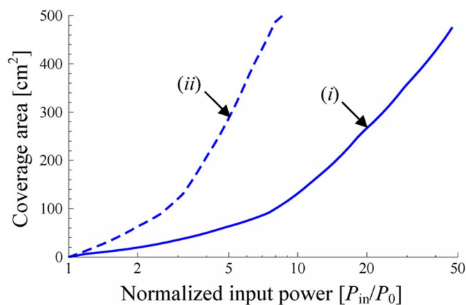
Fig. 8. Interrogation zone coverage area as a function of the normalized input power. (i) With wire grid; (ii) without wire grid.
