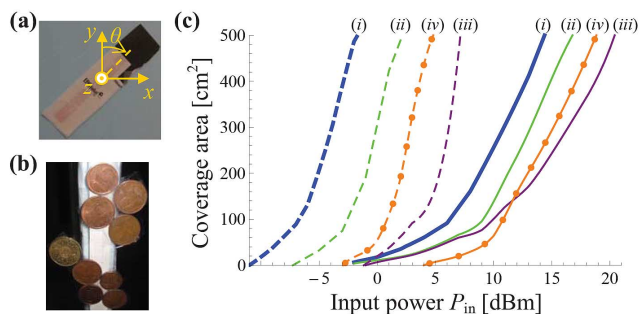
Fig. 9. (a) Photo of the rotated RFID tag. (b) Photo of the RFID tag obstructed by the presence of coins. (c) Coverage areas as a function of the input power in dBm. Solid curves: with wire grid; dashed curves: without wire grid. (i) Results for the unperturbed system, i.e., for the scenario where the RFID tag is y -oriented ( \theta = 0^\circ ) and there are no coins obstructing it; (ii), and (iii) results for different orientations of the RFID tag, \theta = 45^\circ , and \theta = 70^\circ , respectively. (iv) Results for the scenario where the RFID tag is obstructed by coins.
