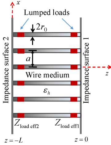
Fig. 1. Geometry of a 2-D WM structure with the wires connected to impedance surfaces through lumped impedance insertions.
