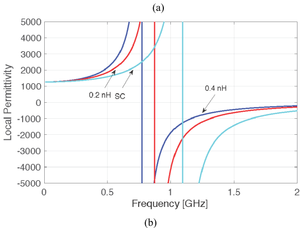
Fig. 5. (a) Local thickness-dependent permittivity of the WM slab with the vias connected to the metallic patches and to the ground plane through the lumped loads and (b) same at low frequencies for the cases with SC and inductive lumped loads demonstrating very large values of the local permittivity even in the static limit. The various lumped loads correspond to those in Fig. 4.
