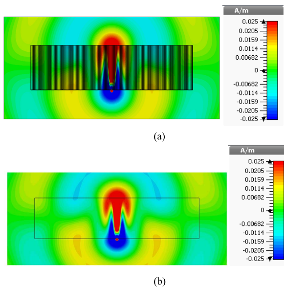
Fig. 15. Numerical simulations of the magnetic-field distribution for (a) true physical WM slab and (b) homogenized local anisotropic material excited by a magnetic line source.
