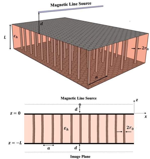
Fig. 12. Geometry of a WM slab loaded by graphene sheets at the WM interfaces and excited by a magnetic line source.
