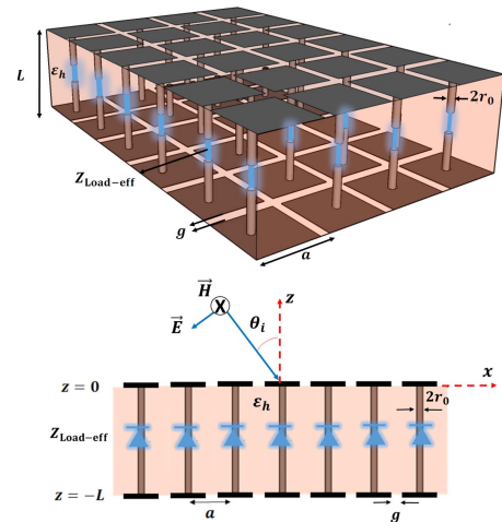
Fig. 7. Geometry of a two-sided mushroom structure with the vias connected to p-i-n diodes with an obliquely incident TM-polarized plane wave.
