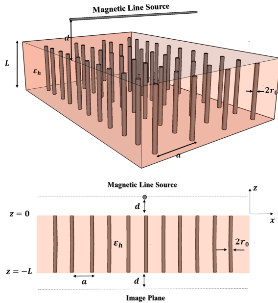
Fig. 9. Geometry of a WM slab excited by a magnetic line source.
