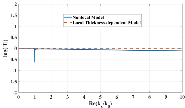
Fig. 10. Transmission response (in logarithmic units) of a WM slab for evanescent waves excited by a magnetic line source. The dimensions of the structure are: a = 215 nm, r_0 = 21.5 nm, L = 7894 nm, and \epsilon_h = 1 .
