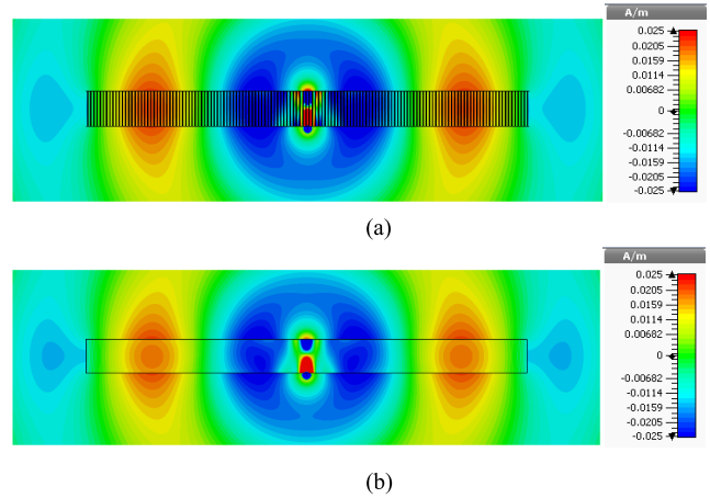
Fig. 17. Numerical simulations of the magnetic-field distribution for (a) true physical WM slab loaded with graphene sheets and (b) homogenized local anisotropic material loaded with graphene sheets and excited by a magnetic line source.
