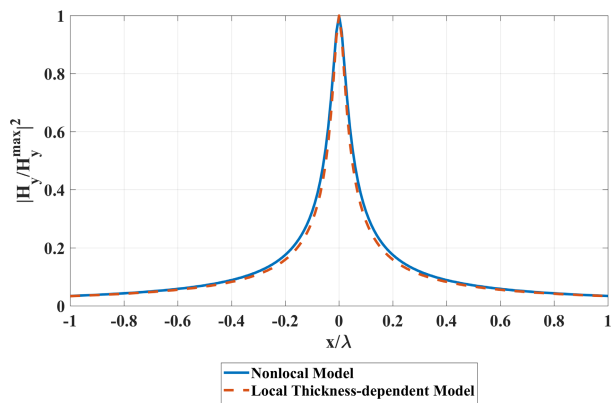
Fig. 11. Square normalized amplitude of the magnetic field at the image plane as a function of x/\lambda at the operating frequency of 19 THz for a WM slab excited by a magnetic line source.
