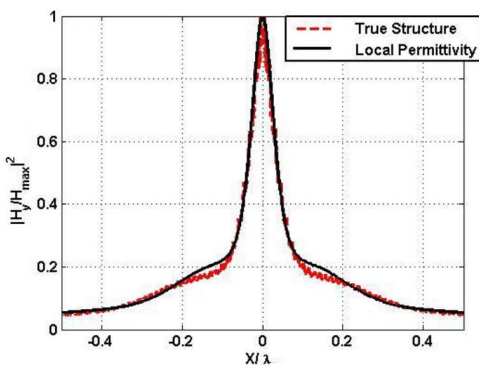
Fig. 16. Square normalized amplitude of the magnetic field at the image plane for a true physical WM slab and homogenized local anisotropic slab excited by a magnetic line source.
