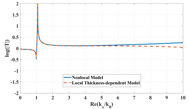
Fig. 13. Transmission response (in logarithmic units) of a WM slab loaded with graphene sheets for the evanescent waves due to a magnetic line source excitation. The dimensions of the WM slab and graphene parameters are: a = 215 nm, r_0 = 21.5 nm, L = 2400 nm, \epsilon_h = 1 , T = 300 K, \tau = 0.5 ps, and \mu_c = 1.5 eV.
