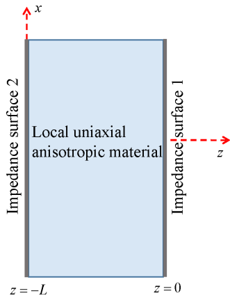
Fig. 2. Local uniaxial anisotropic material with impedance surfaces at the interfaces as an equivalent geometry to the WM structure presented in Fig. 1.
