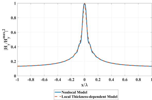
Fig. 14. Square normalized amplitude of the magnetic field at the image plane as a function of x/\lambda at the operating frequency of 19 THz for a WM slab loaded with graphene sheets at the WM interfaces and excited by a magnetic line source.
