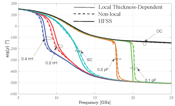
Fig. 4. Phase of the reflection coefficient for a mushroom structure with the vias connected to the ground through inductive and capacitive loads (including the cases of SC and OC). The dimensions of the structure are: a = 2 mm, g = 0.2 mm, r_0 = 0.05 mm, L = 1 mm, \epsilon_h = 10.2 , and \theta_i = 60^\circ . The load is connected to the ground through a gap of 0.1 mm with the parasitic capacitance C_{\text{par}} \approx 0.02 pF and parasitic inductance L_{\text{par}} \approx 0.06 nH (estimated by curve fitting).
