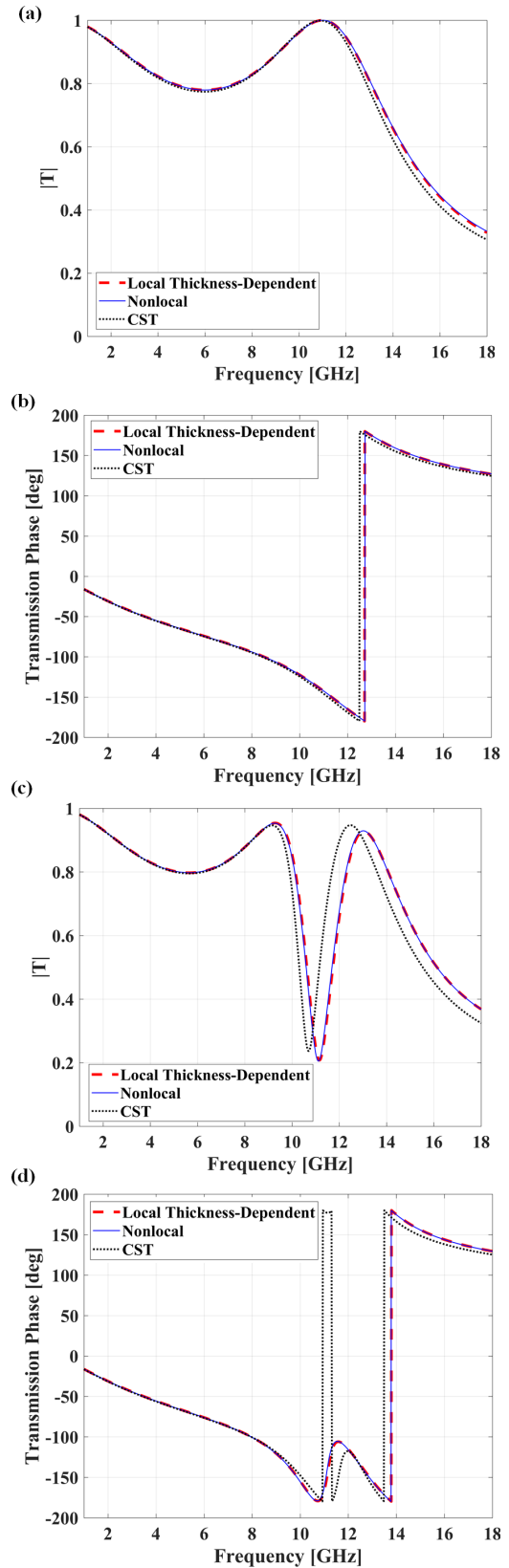
Fig. 8. Transmission response (magnitude and phase) of the two-sided mushroom structure with the vias connected to p-i-n diodes in the middle of the WM slab in (a) and (b) OFF, and (c) and (d) ON states under illumination of an obliquely incident TM-polarized plane wave. The dimensions of the structure are: a = 2 mm, g = 0.2 mm, r_0 = 0.05 mm, L = 2 mm, \epsilon_h = 10.2 , and \theta_i = 60^\circ .
