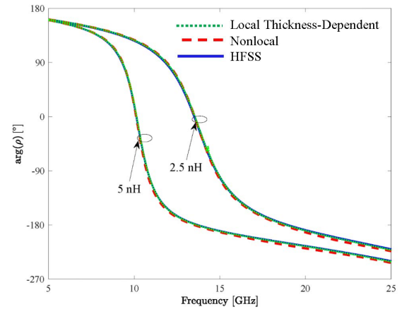
Fig. 6. Phase of the reflection coefficient for the air-filled mushroom structure with the vias connected to the ground plane through inductive loads (2.5 and 5 nH) (with the geometry in Fig. 3). The dimensions of the structure are: a = 2 mm, g = 0.2 mm, r_0 = 0.05 mm, L = 1 mm, \epsilon_h = 1 , and \theta_i = 45^\circ .
