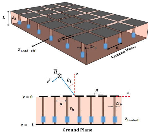
Fig. 3. Geometry of a mushroom high-impedance surface with loaded vias with an obliquely incident TM-polarized plane wave.
