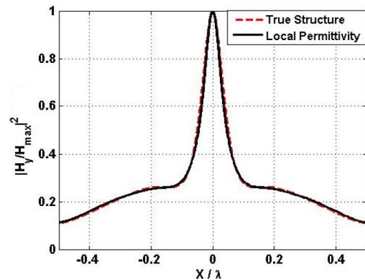
Fig. 18. Square normalized amplitude of the magnetic field at the image plane for a true physical WM slab with graphene sheets and homogenized local anisotropic slab with graphene sheets excited by a magnetic line source.
