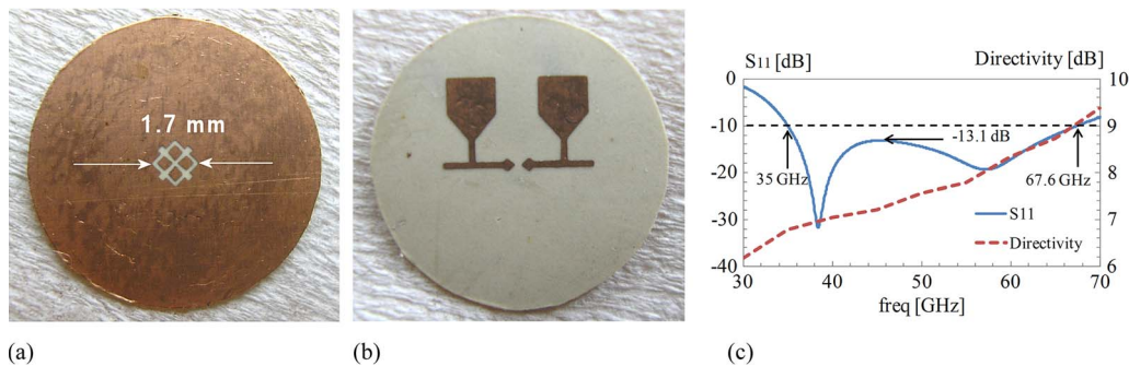
Figure 2. XETS prototype for 30–70 GHz operation when integrated with a MACOR lens. Photographs of the (a) front face and (b) back face. (c) Simulated input reflection coefficient and directivity when radiating into unbounded MACOR.
