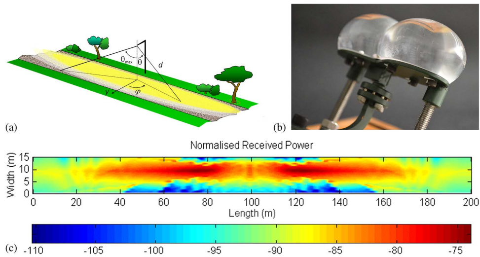
Figure 11. (a) Geometry of a street sectored cell. (b) Photograph of a shaped lens antenna for a constant flux illumination of the street at 60 GHz. (c) Received power within the cell limits for a transmitted power of 22 dBm.
