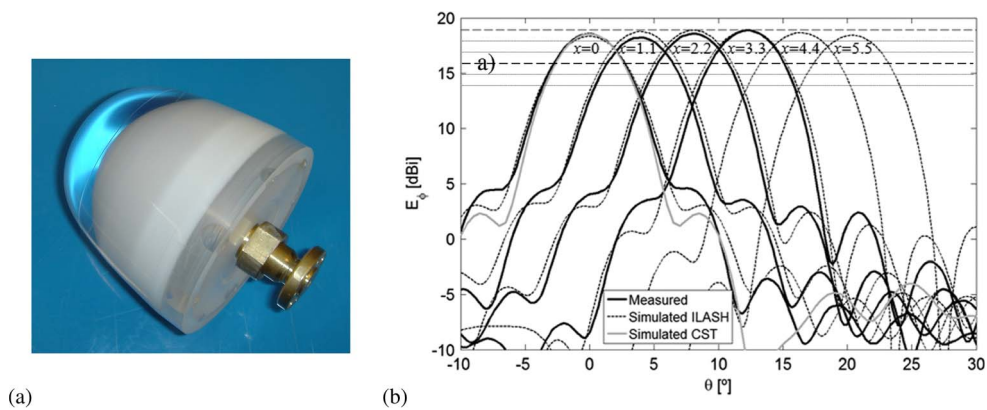
Figure 13. (a) Fabricated MACOR/acrylic lens prototype, showing the attached 60-GHz band waveguide feed. (b) Simulated and measured gain radiation patterns at 62.5 GHz, in the H-plane, with feed at 0, 1.1, 2.2, 3.3, 4.4, and 5.5 mm from the lens axis [31].
