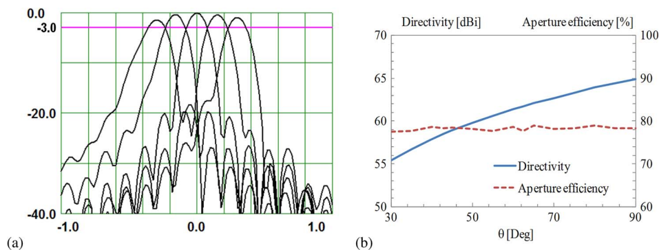
Figure 17. a) Radiation pattern of the reflector when illuminated by the fabricated lens prototype, with an inner shell of MACOR and an outer shell of acrylic. (b) Calculated directivity and aperture efficiency of the reflector for the central beam.
