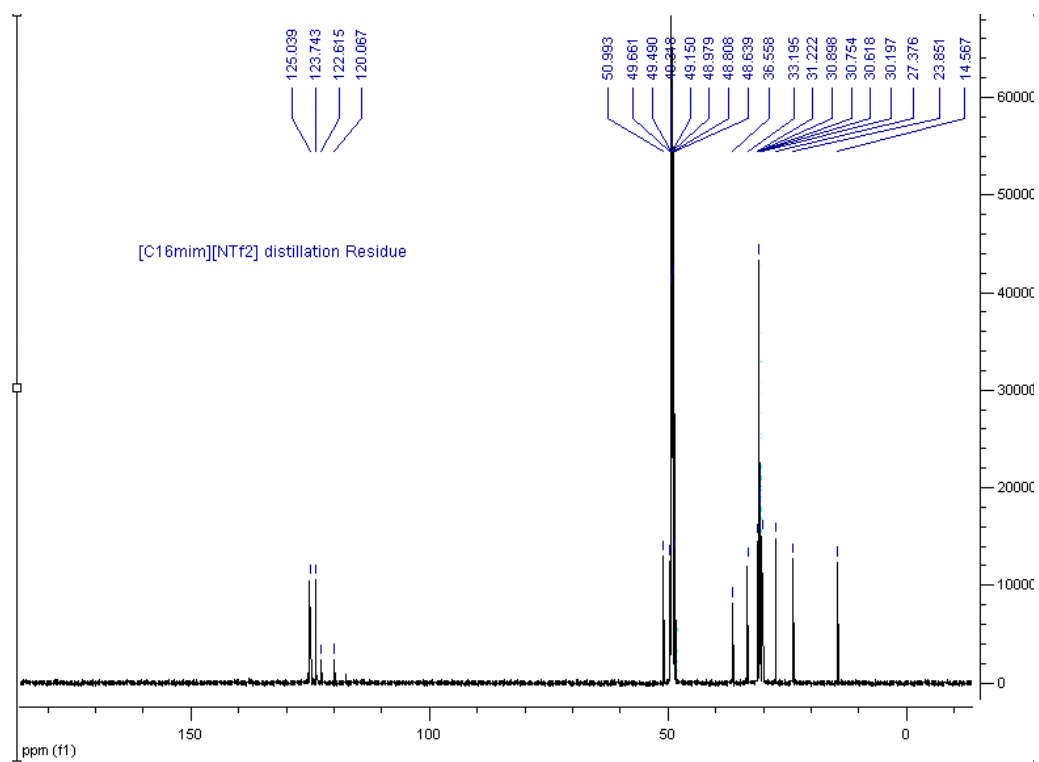
Supplementary Figure 7b. The ^{13}\text{C} NMR spectrum of undistilled [\text{C}_{16}\text{mim}][\text{NTf}_2] after 5 h at 300 °C.
