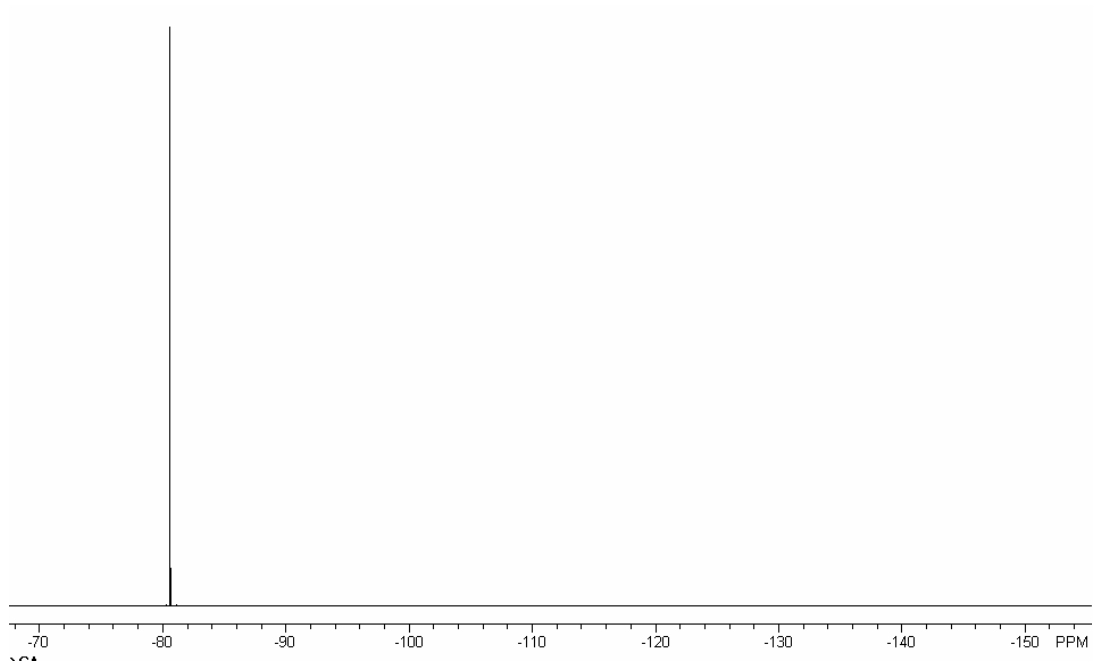
Supplementary Figure 10b. The ^{19}\text{F} NMR spectrum of the undistilled [\text{C}_6\text{mim}][\text{NTf}_2] after 1 h at t = 200\text{ }^\circ\text{C} and p \leq 0.001\text{ mbar} .
