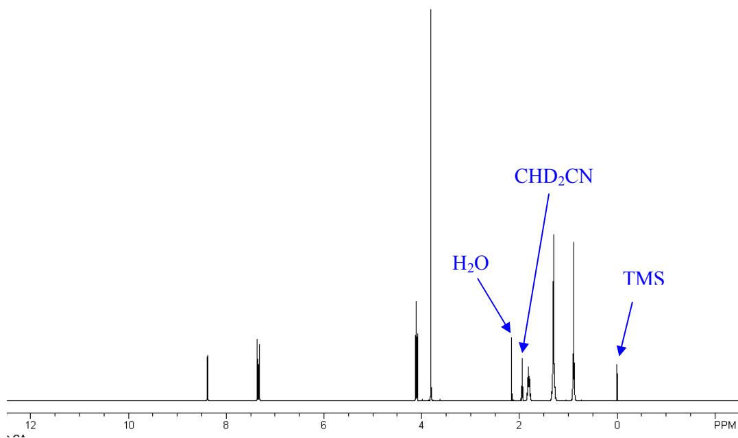
Supplementary Figure 8a. The ^1\text{H} NMR spectrum of original sample of [\text{C}_6\text{mim}][\text{NTf}_2] . The \text{CHD}_2\text{CN} and TMS peaks originate from the NMR solvent.
