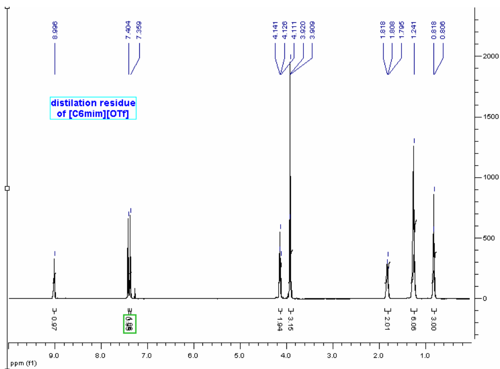
Supplementary Figure 3b. The ^1\text{H} NMR spectrum of undistilled [\text{C}_6\text{mim}][\text{OTf}] after 4 h at 300 °C.
