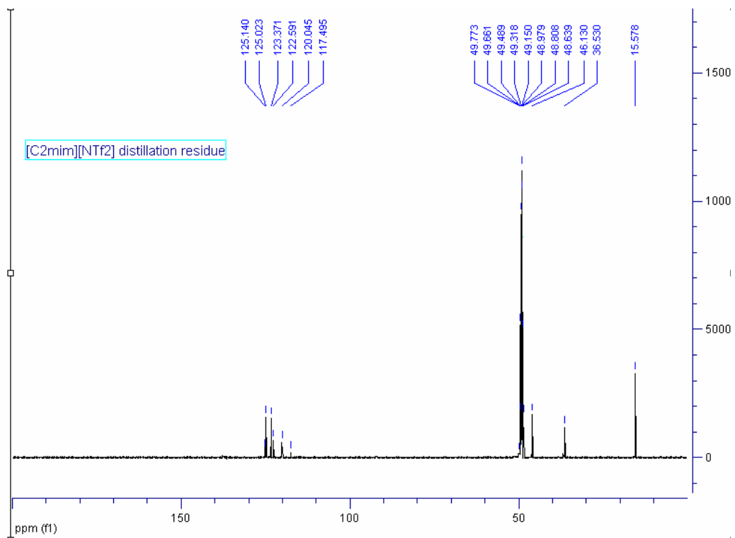
Supplementary Figure 2b. The 13 C NMR spectrum of undistilled [C 2 mim][NTf 2 ] after 5 h at 300 °C
