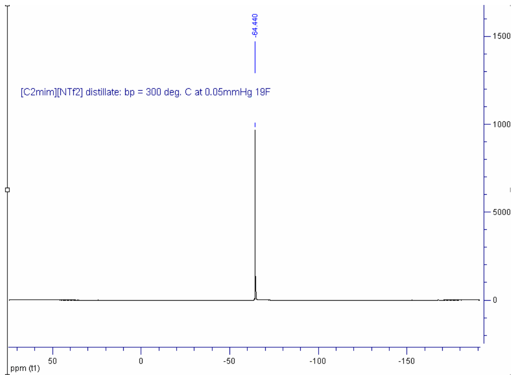
Supplementary Figure 1c. The ^{19}\text{F} NMR spectrum of distilled [\text{C}_2\text{mim}][\text{NTf}_2] after 5 h at 300 °C
