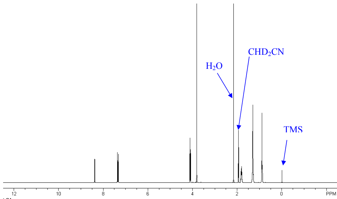
Supplementary Figure 9a. The ^1\text{H} NMR spectrum of the distilled [\text{C}_6\text{mim}][\text{NTf}_2] after 1 h at t = 200\text{ }^\circ\text{C} and p \leq 0.001\text{ mbar} . The larger-than-normal water peak is an artefact of the preparation of the NMR sample. The \text{CHD}_2\text{CN} and \text{TMS} peaks originate from the NMR solvent.
