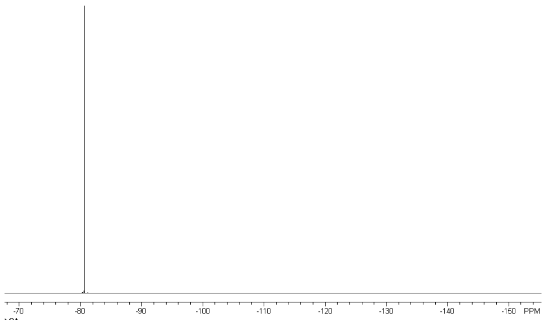
Supplementary Figure 9b. The ^{19}\text{F} NMR spectrum of the distilled [\text{C}_6\text{mim}][\text{NTf}_2] after 1 h at t = 200\text{ }^\circ\text{C} and p \leq 0.001\text{ mbar} .
