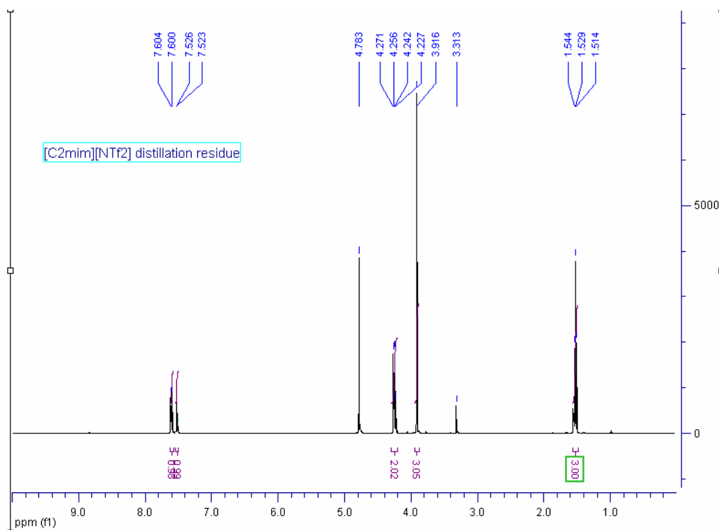
Supplementary Figure 2a. The ^1\text{H} NMR spectrum of undistilled [\text{C}_2\text{mim}][\text{NTf}_2] after 5 h at 300\text{ }^\circ\text{C}
