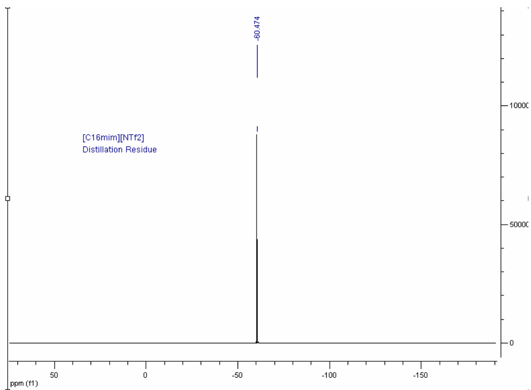
Supplementary Figure 7c. The ^{19}\text{F} NMR spectrum of undistilled [\text{C}_{16}\text{mim}][\text{NTf}_2] after 5 h at 300 °C.
