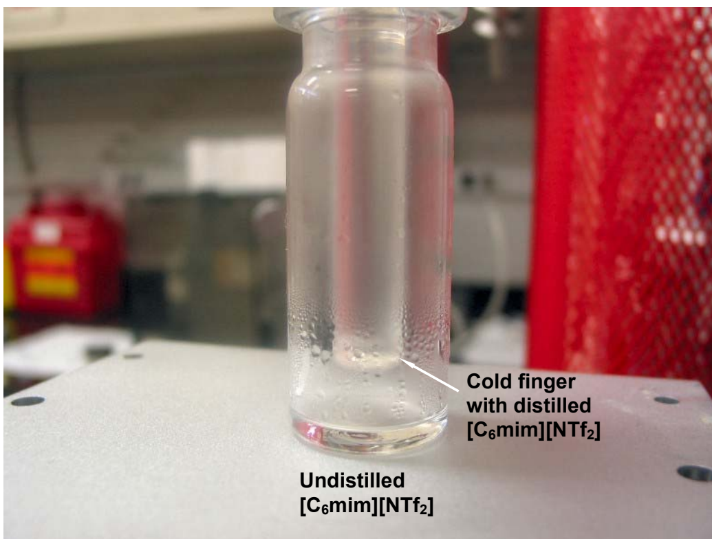
Supplementary Figure 14. A picture of the sublimation apparatus at the end of the distillation experiment with [C 6 mim][NTf 2 ] at \leq 0.001 mbar. After an hour at 200 °C, large beads of liquid had formed on the cold finger and on the lower wall of the flask; the liquid in the flask was still clear and colourless to the eye.
