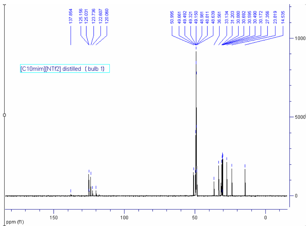
Supplementary Figure 4b. The ^{13}\text{C} NMR spectrum of distilled [\text{C}_{10}\text{mim}][\text{NTf}_2] after 5 h at 300 °C.
