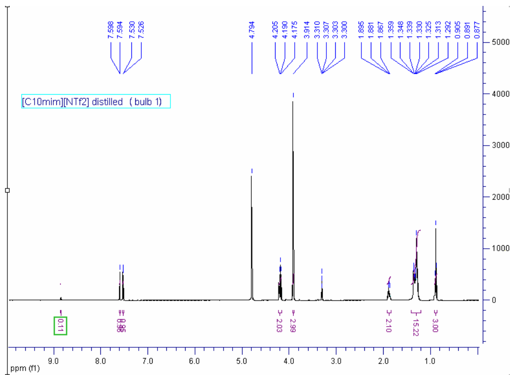
Supplementary Figure 4a. The ^1\text{H} NMR spectrum of distilled [\text{C}_{10}\text{mim}][\text{NTf}_2] after 5 h at 300\text{ }^\circ\text{C}
