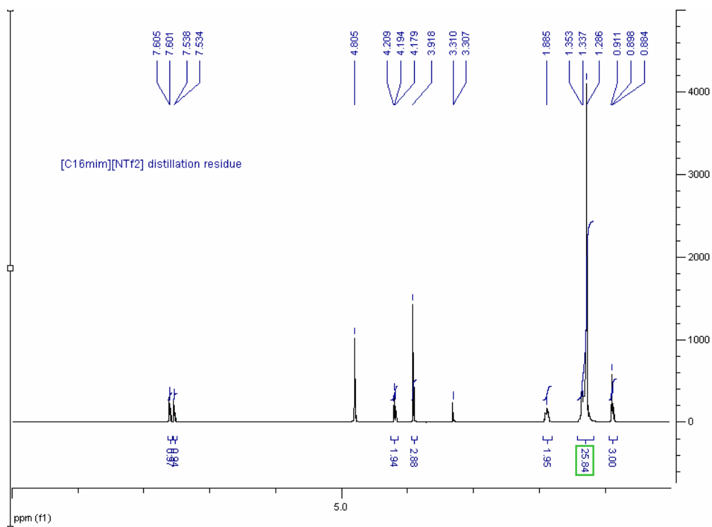
Supplementary Figure 7a. The ^1\text{H} NMR spectrum of undistilled [\text{C}_{16}\text{mim}][\text{NTf}_2] after 5 h at 300 °C.
