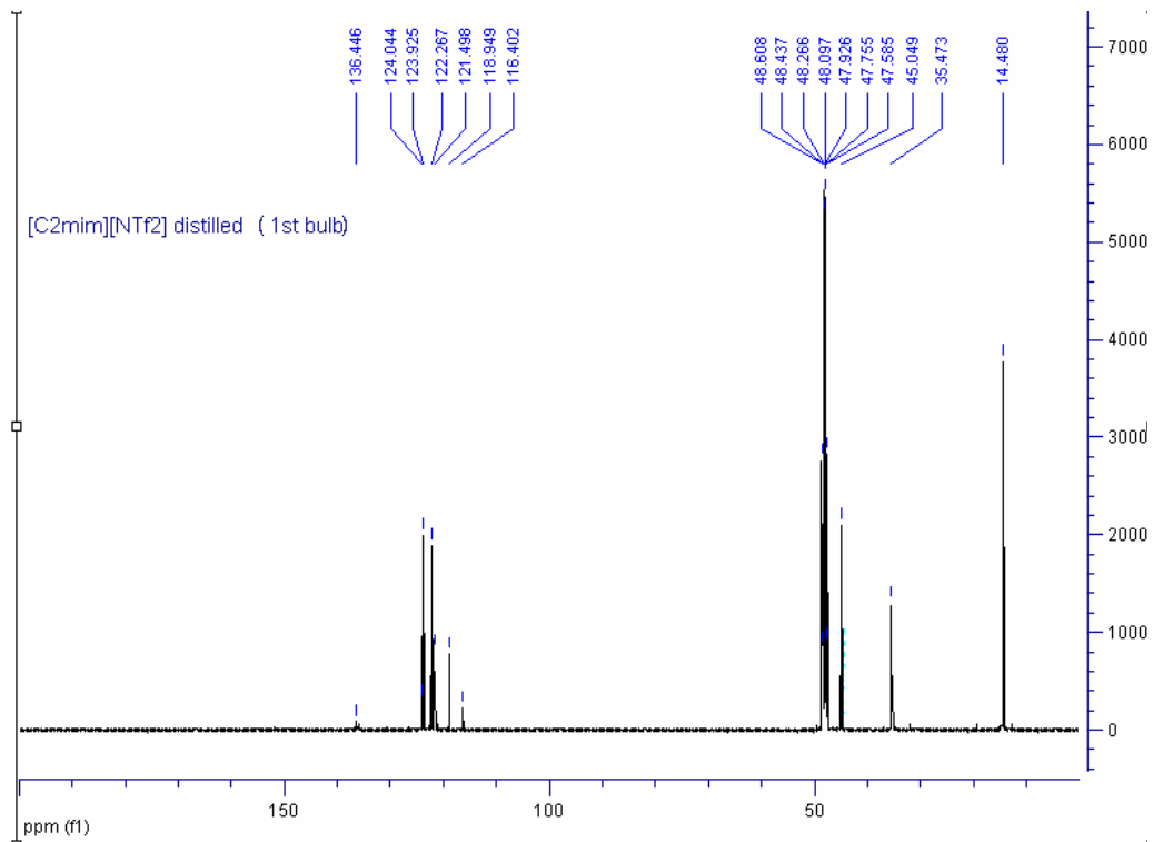
Supplementary Figure 1b. The 13 C NMR spectrum of distilled [C 2 mim][NTf 2 ] after 5 h at 300 °C
