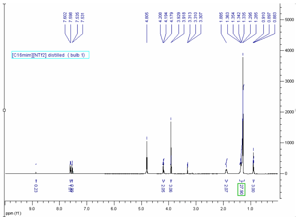
Supplementary Figure 6a. The ^1\text{H} NMR spectrum of distilled [\text{C}_{16}\text{mim}][\text{NTf}_2] after 5 h at 300 °C.
