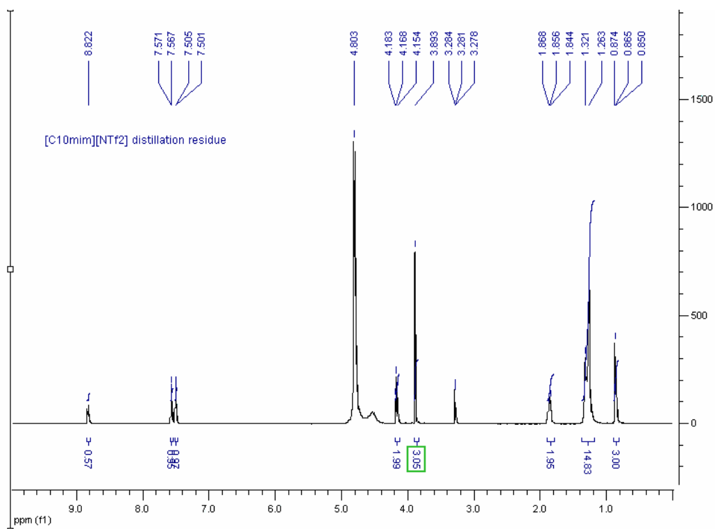
Supplementary Figure 5a. The 1 H NMR spectrum of undistilled [C 10 mim][NTf 2 ] after 5 h at 300 °C
