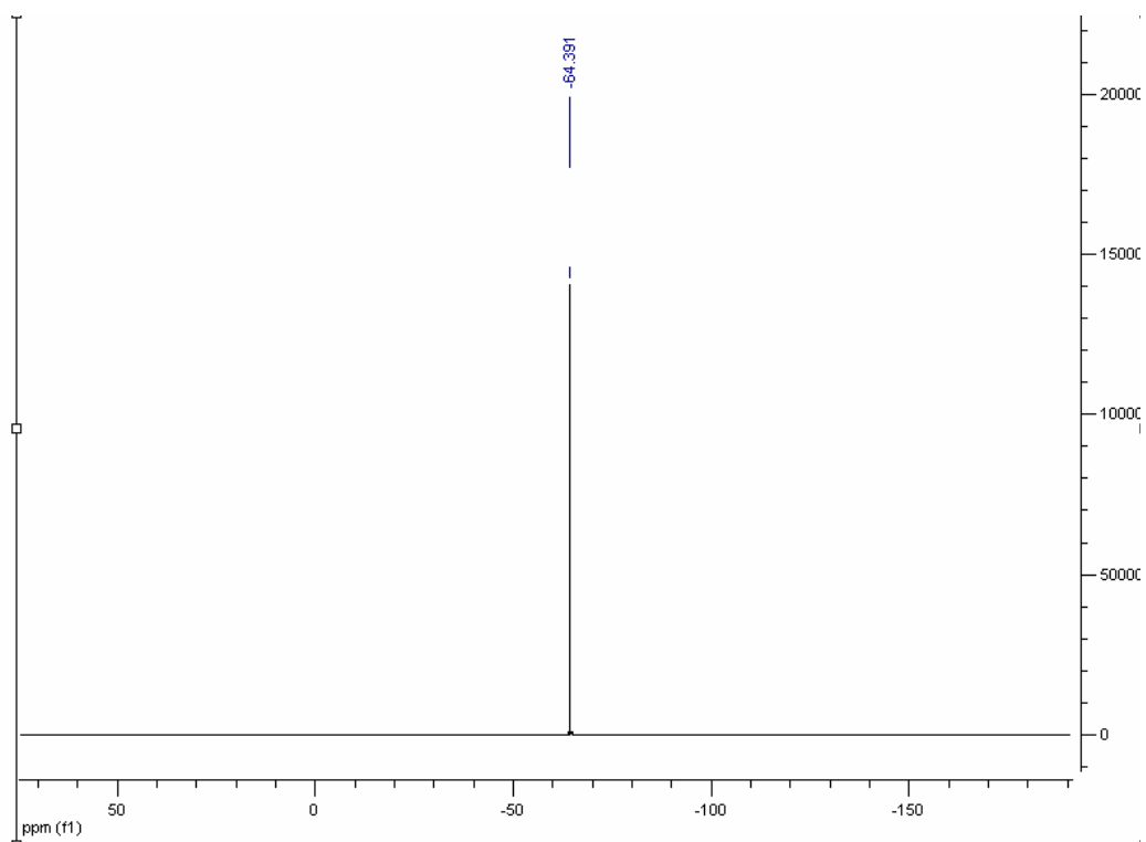
Supplementary Figure 6c. The ^{19}\text{F} NMR spectrum of distilled [\text{C}_{16}\text{mim}][\text{NTf}_2] after 5 h at 300 °C.
