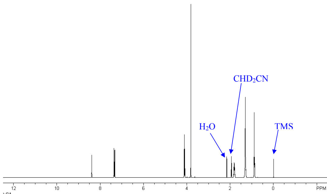
Supplementary Figure 10a. The ^1\text{H} NMR spectrum of the undistilled [\text{C}_6\text{mim}][\text{NTf}_2] after 1 h at t = 200\text{ }^\circ\text{C} and p \leq 0.001\text{ mbar} . The \text{CHD}_2\text{CN} and TMS peaks originate from the NMR solvent.
