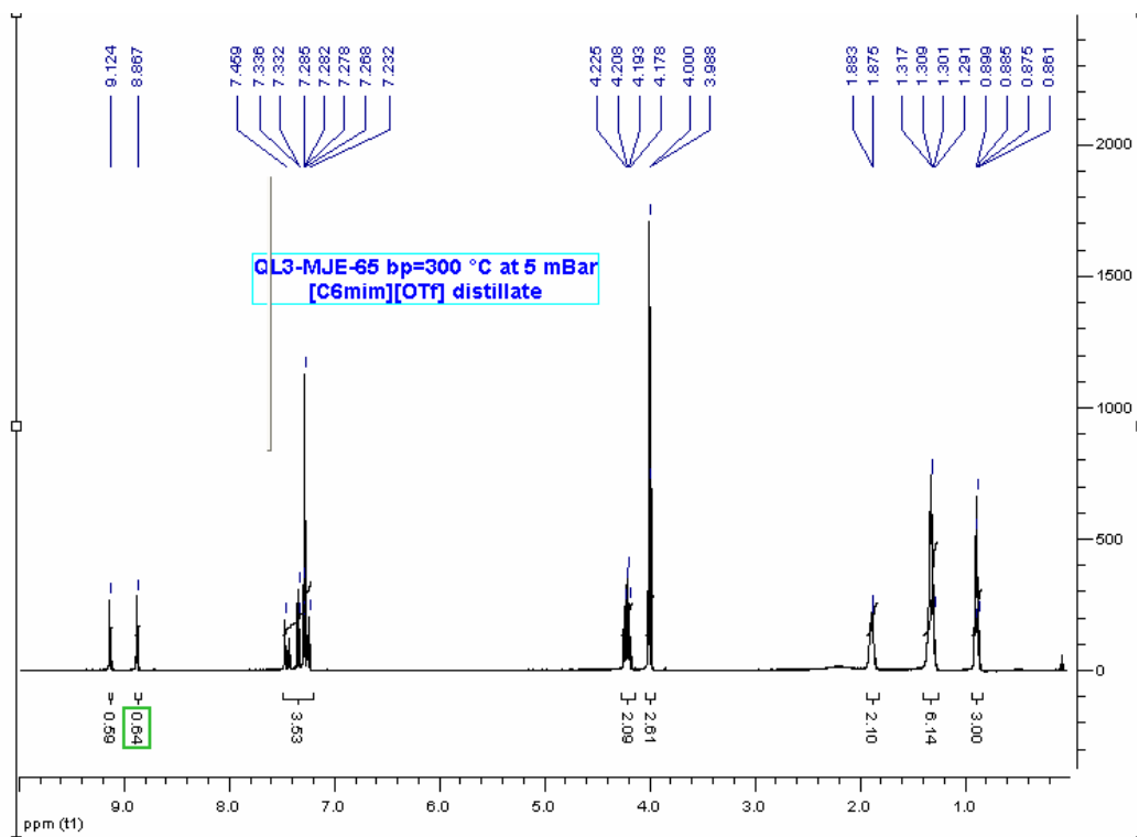
Supplementary Figure 3a. The ^1\text{H} NMR spectrum of distilled [\text{C}_6\text{mim}][\text{OTf}] after 4 h at 300 °C.
