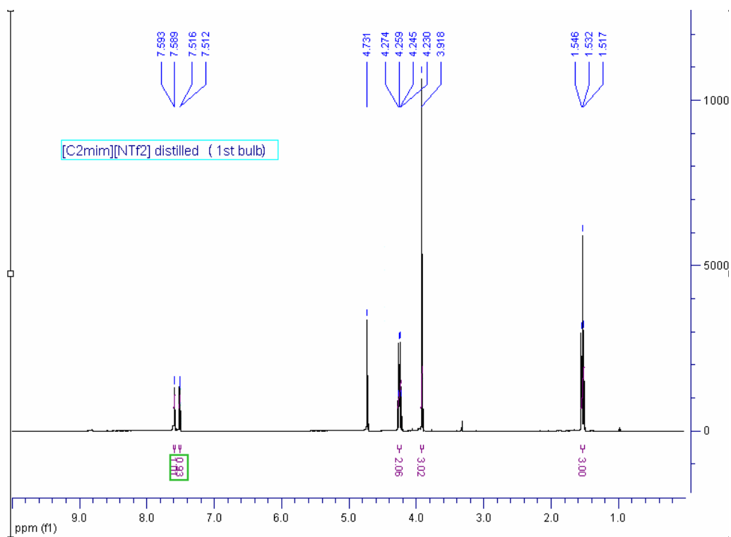
Supplementary Figure 1a. The 1 H NMR spectrum of distilled [C 2 mim][NTf 2 ] after 5 h at 300 °C
