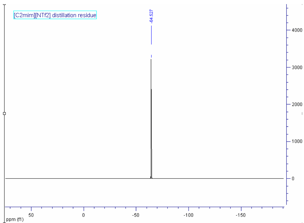
Supplementary Figure 2c. The ^{19}\text{F} NMR spectrum of undistilled [\text{C}_2\text{mim}][\text{NTf}_2] after 5 h at 300 °C
