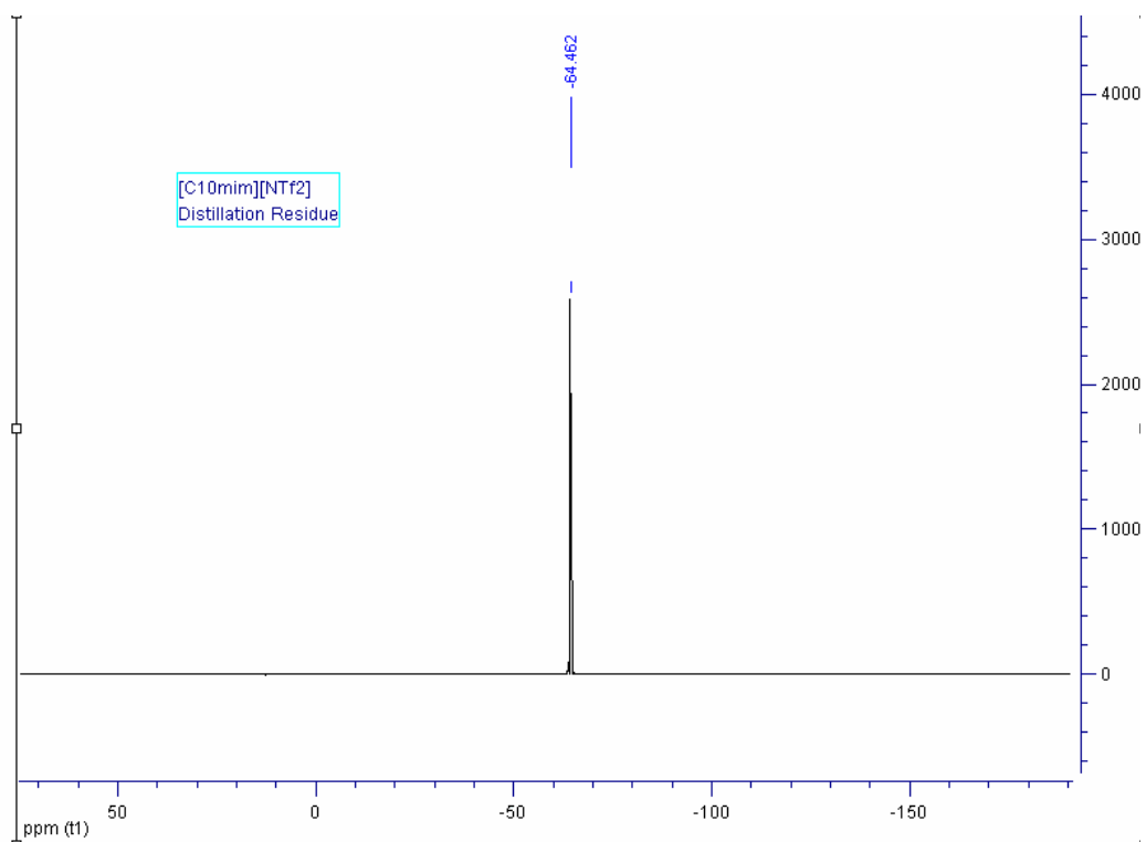
Supplementary Figure 5c. The ^{19}\text{F} NMR spectrum of undistilled [\text{C}_{10}\text{mim}][\text{NTf}_2] after 5 h at 300 °C.
