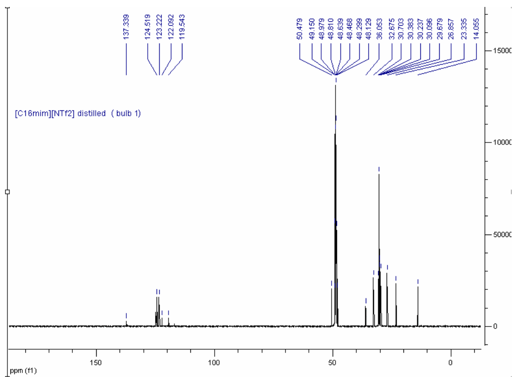
Supplementary Figure 6b. The ^{13}\text{C} NMR spectrum of distilled [\text{C}_{16}\text{mim}][\text{NTf}_2] after 5 h at 300 °C.
