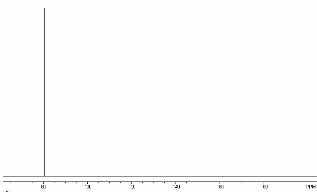
Supplementary Figure 8b. The ^{19}\text{F} NMR spectrum of original sample of [\text{C}_6\text{mim}][\text{NTf}_2] .
