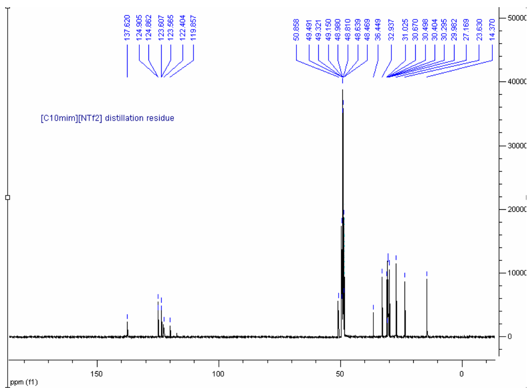
Supplementary Figure 5b. The ^{13}\text{C} NMR spectrum of undistilled [\text{C}_{10}\text{mim}][\text{NTf}_2] after 5 h at 300 °C.
