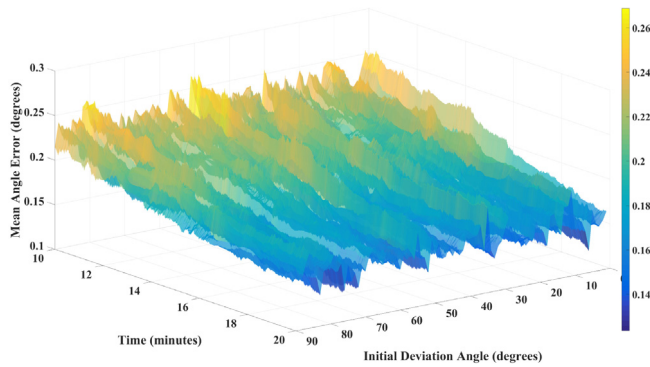
Fig. 8. Steady state mean of \tilde{\theta}(t) for t \geq 10 minutes.
