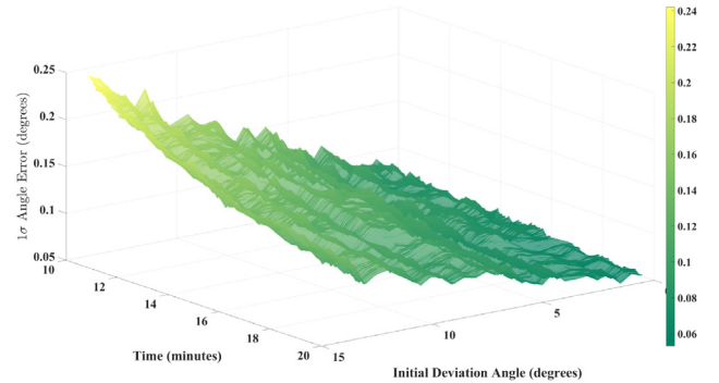
Fig. 4. Steady state standard deviation of \tilde{\theta}(t) for t \ge 10 minutes (local evaluation).
