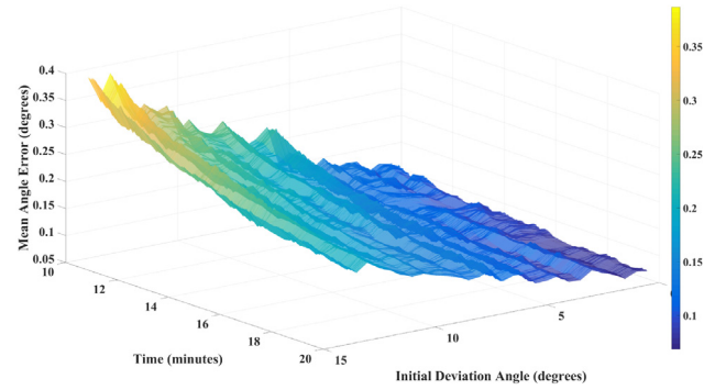
Fig. 3. Steady state mean of \tilde{\theta}(t) for t \ge 10 minutes (local evaluation).
