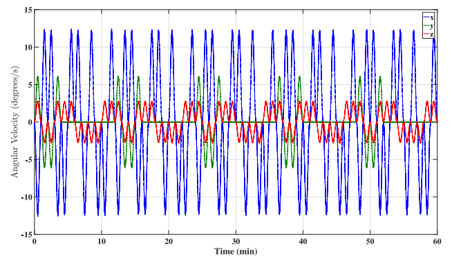
Fig. 11. MRT angular velocity on body-frame.
