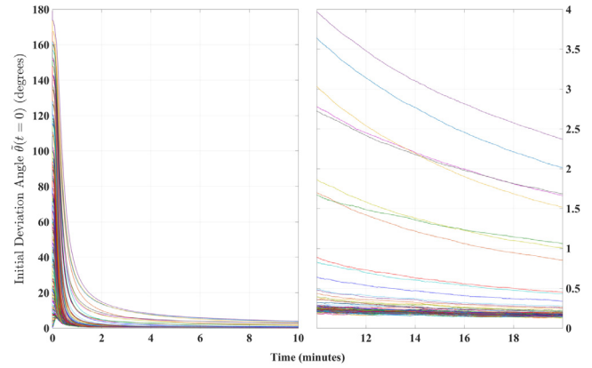
Fig. 7. Time evolution of \tilde{\theta}(t) for \tilde{\theta}(0) = 1, 2, \dots, 179 degrees.
