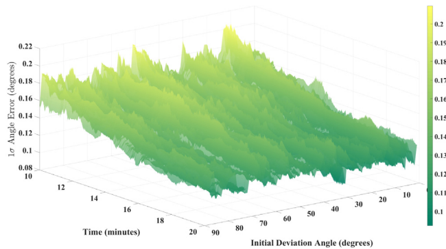
Fig. 9. Steady state standard deviation of \tilde{\theta}(t) for t \geq 10 minutes.
