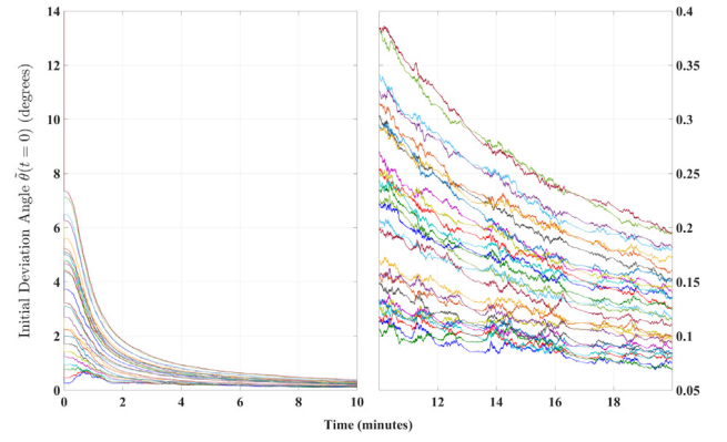
Fig. 2. Time evolution of \tilde{\theta}(t) for \tilde{\theta}(0) = 0.5 \dots 14 degrees (local evaluation).
