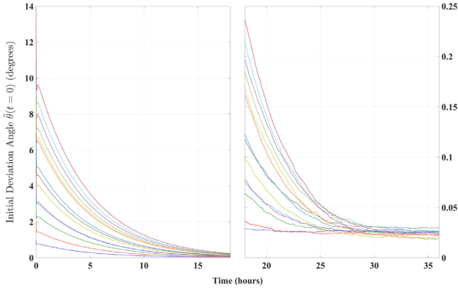
Fig. 5. Time evolution of \tilde{\theta}(t) for \tilde{\theta}(0) = 1, 2 \dots 14 degrees (local evaluation with \tilde{\mathbf{p}}(t) = \mathbf{0} ).
