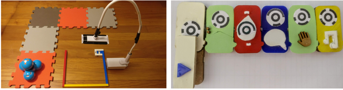
Fig. 2. Left) the ACCemby setup: the map, Dash robot, workspace and tripod with mobile device to identify blocks. Right) an example of a sequence of blocks to repeat the instructions moving forward and saying "hi" two times, and then dancing. The white Play block is at the beginning of the sequence, and the green Loop blocks marks the start and end of the instructions to repeat.
